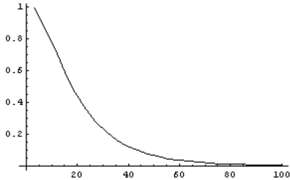
Diagram 3: Probability of obtaining a special majority of at least 2/3 conditional on X=1 where p(n) = 1/(1+\exp(-k/n)) with k=10
