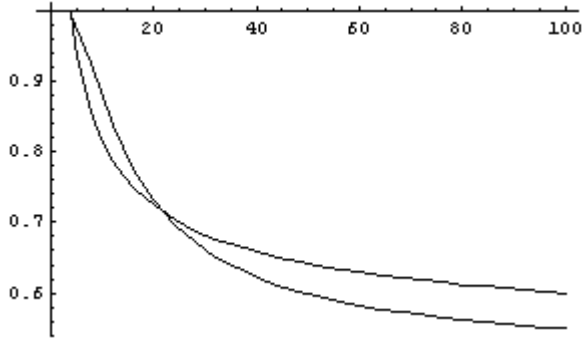
Diagram 2: 1/(1+\exp(-20/n)) (the lower one of the two curves for larger values of n ) and 1/2 + 1/n^{0.4999} (the higher one of the two curves for larger values of n )
